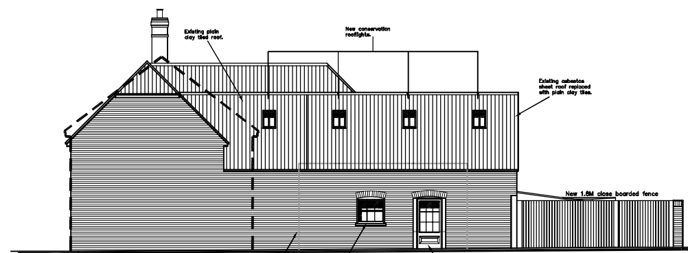
NORTH
