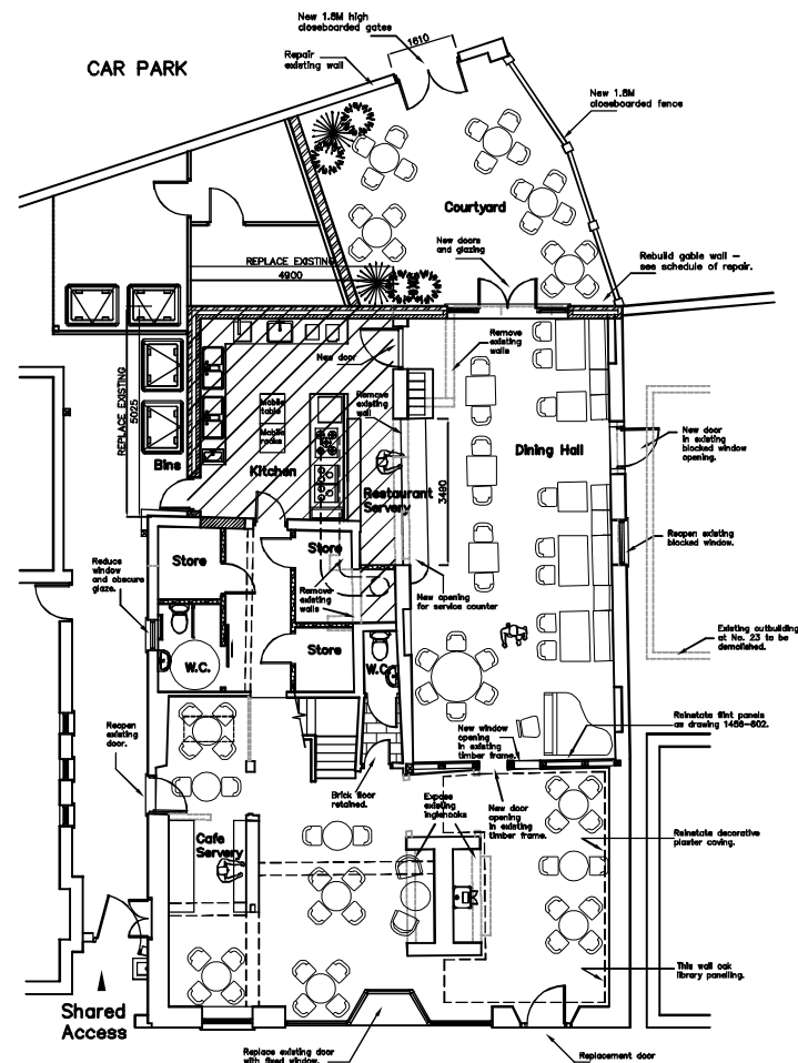
GROUND FLOOR
