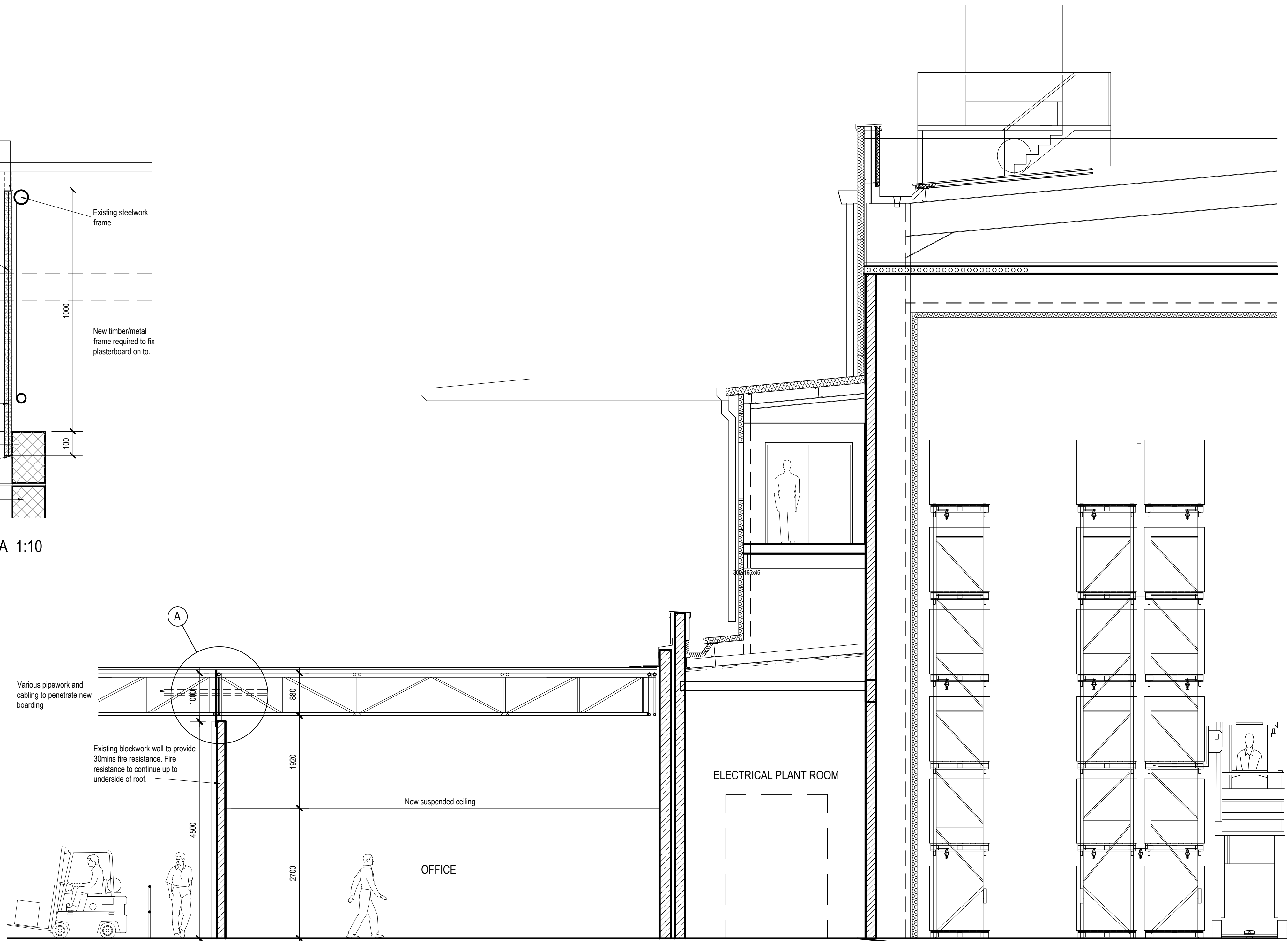
SECTION B - B 1:50
