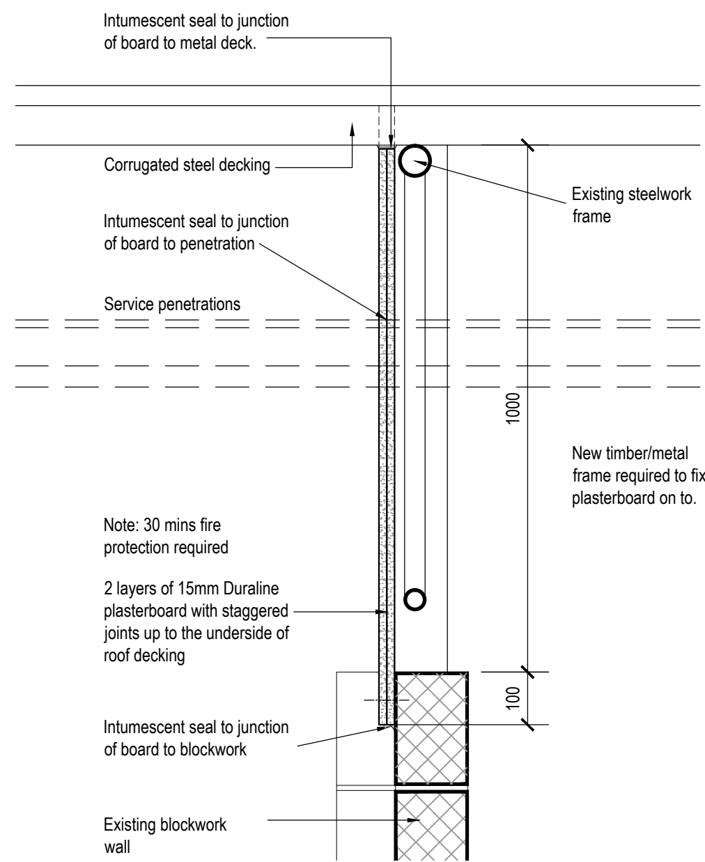
DETAIL A 1:10
