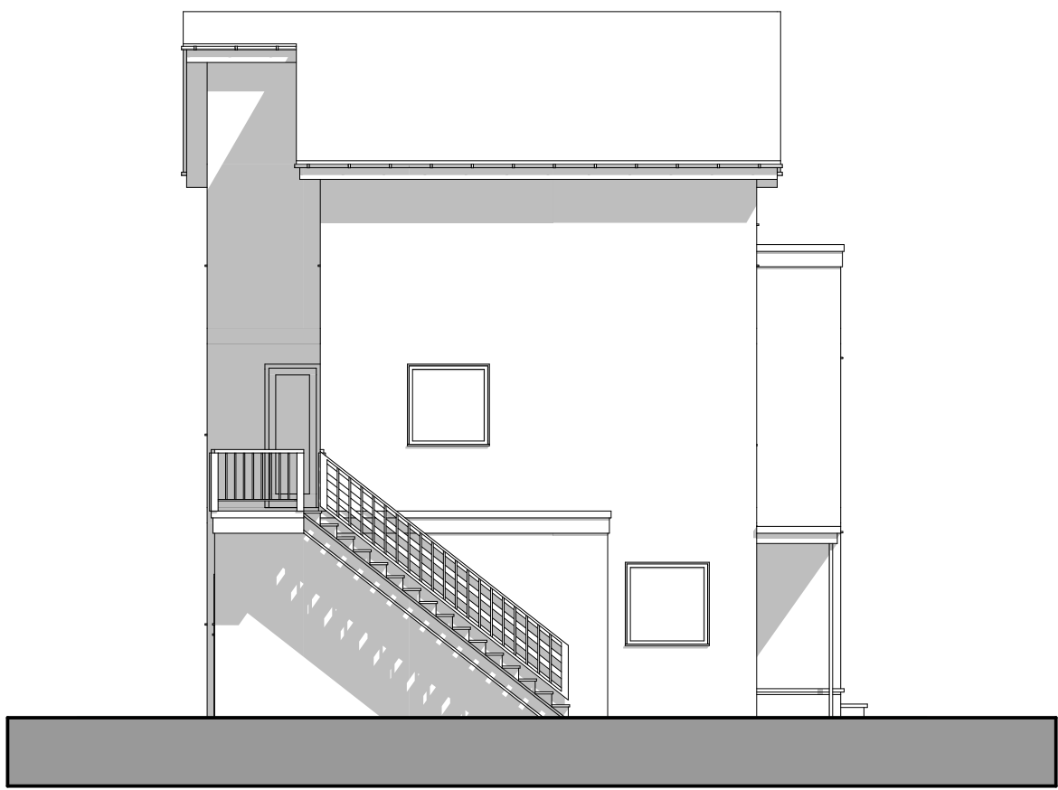
Existing West Elevation 1:100
