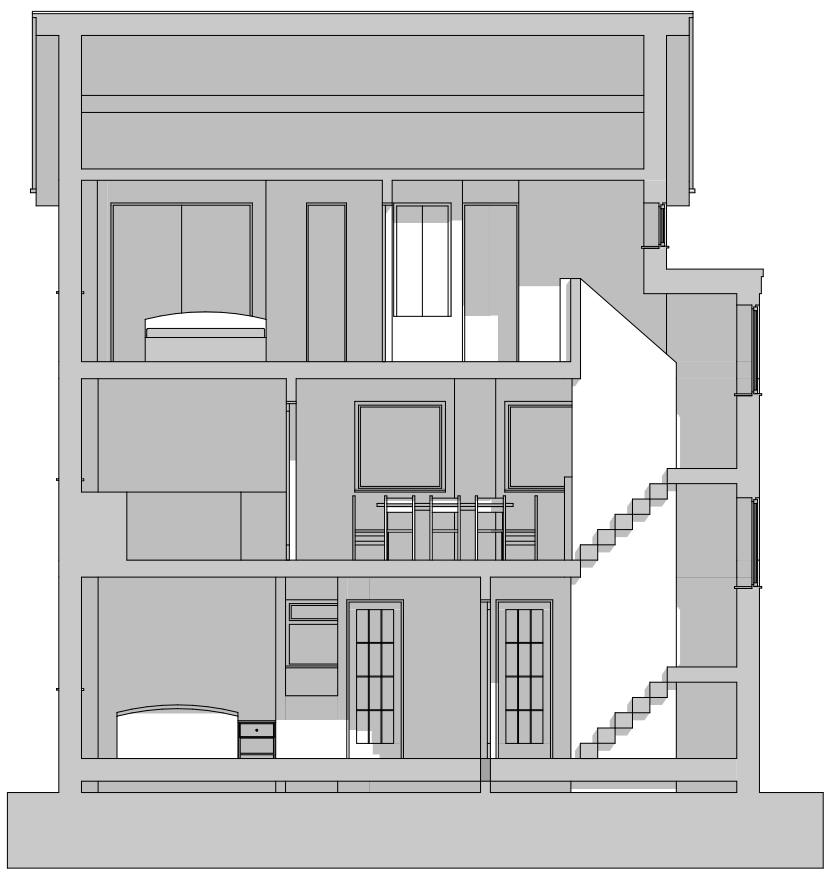
Existing Section S-2 1:100
