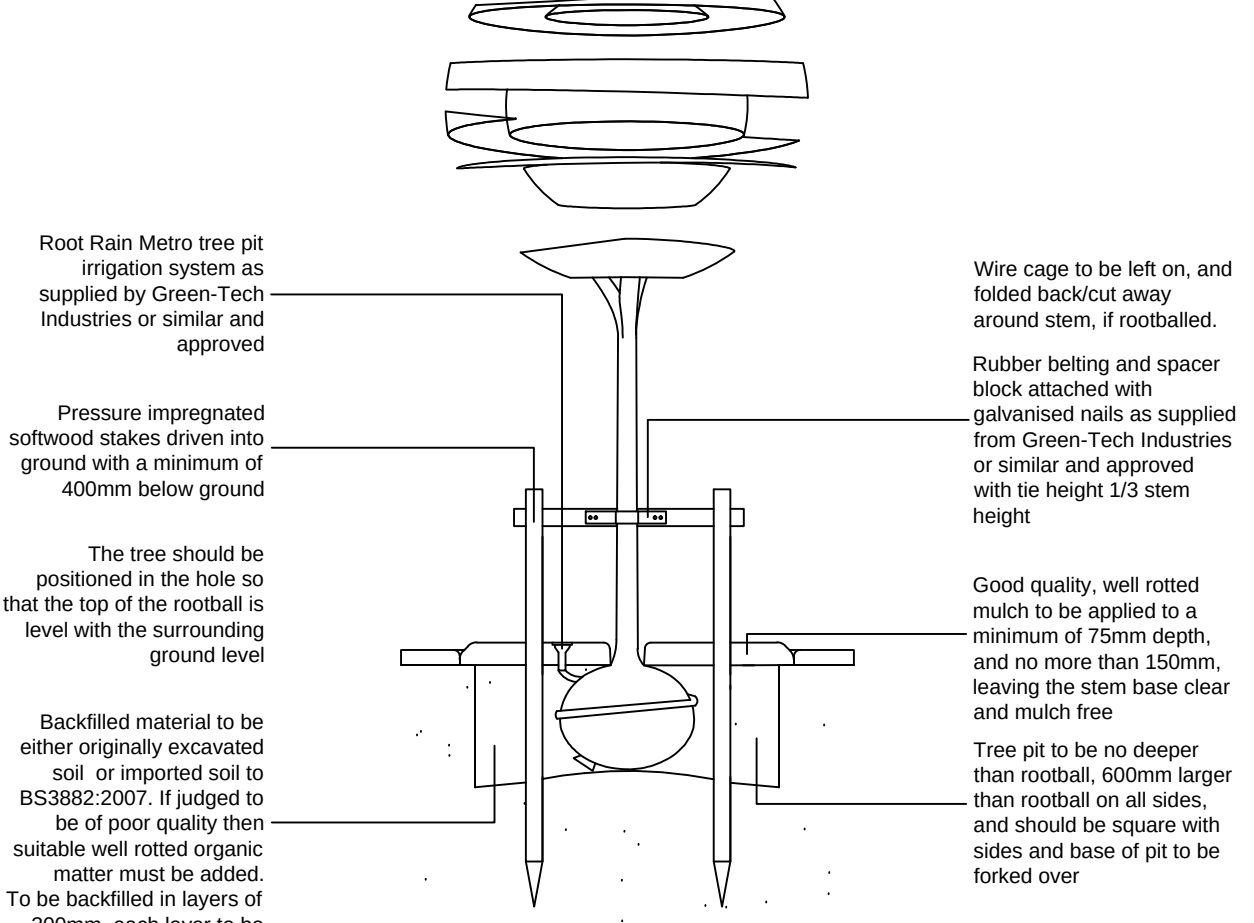
Tree Planting Pit Detail within Soft Landscape
