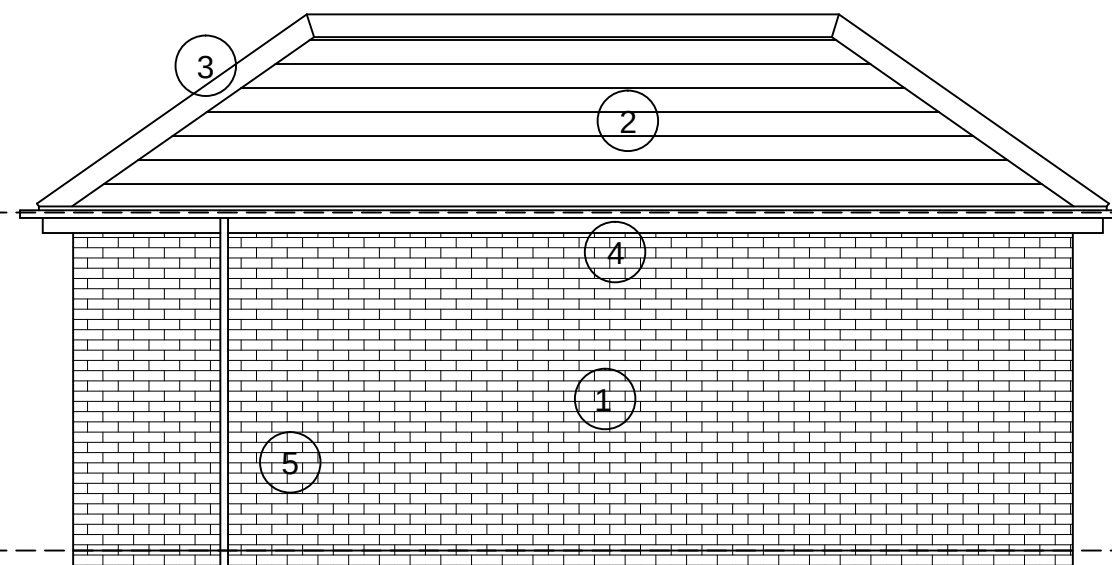
NORTH ELEVATION (1:50)
