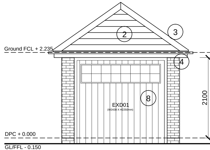
EAST ELEVATION (1:50)
