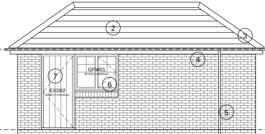
SOUTH ELEVATION (1:50)
