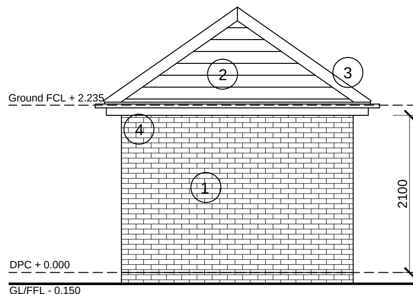
WEST ELEVATION (1:50)
