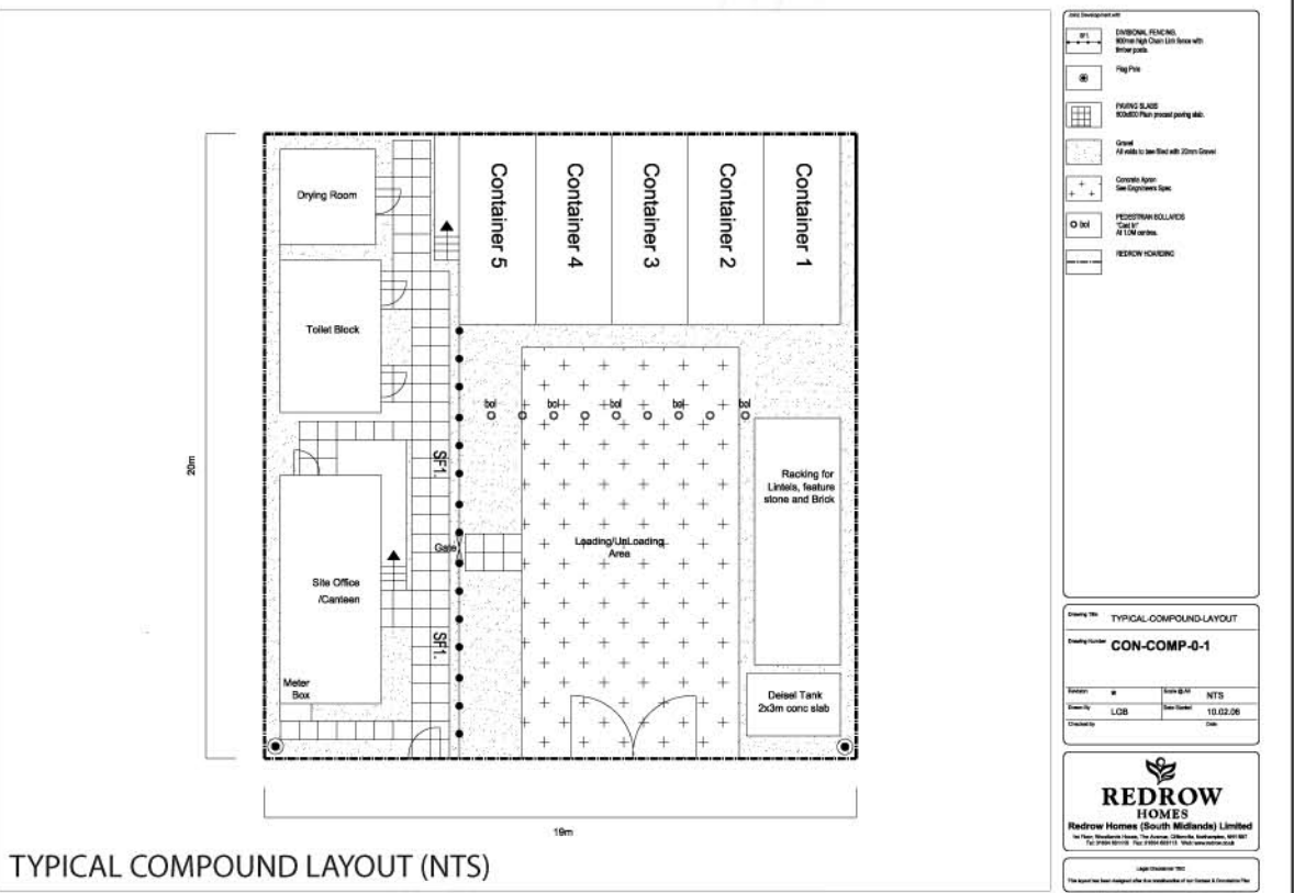
TYPICAL COMPOUND LAYOUT (NTS)
