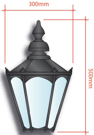
Item 5. Half Stratford (4 off) Half Stratford lantern in Black. SCALE 1:10 @ A3
