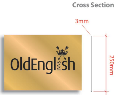
Item 2. (1 off) 350mm x 250mm replacement brass plaque. Scale 1:10 @ A3 AGL:1440mm
