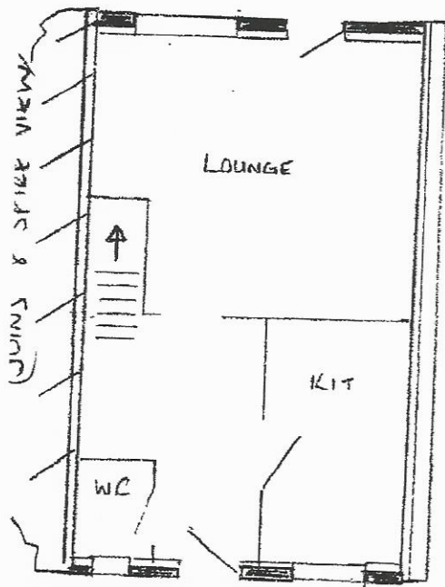
EXISTING GROUND
