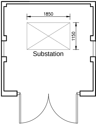
Floor Plan
