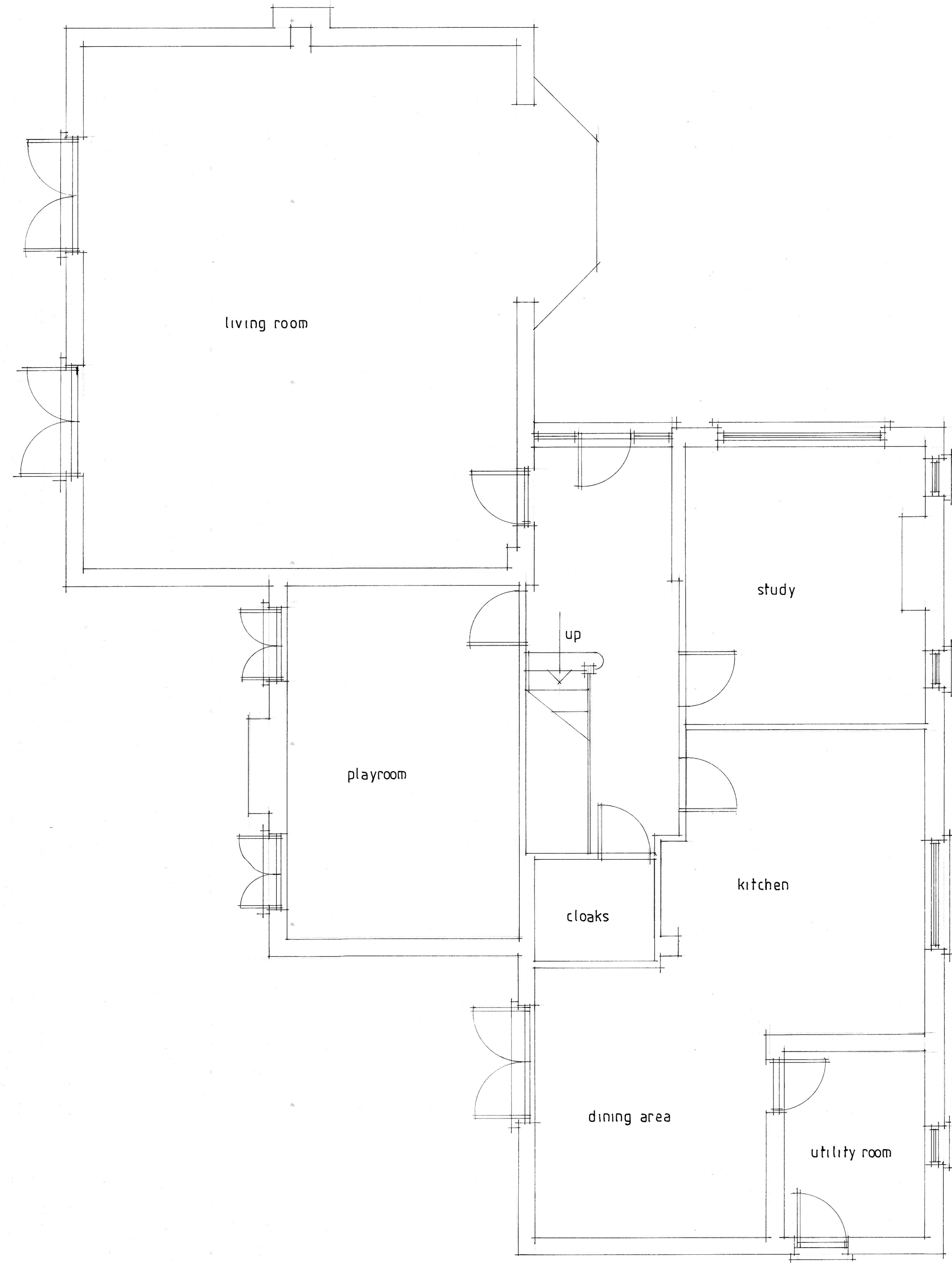
existing ground floor
