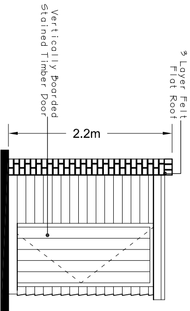
Front Elevation @ 1:50 Scale
