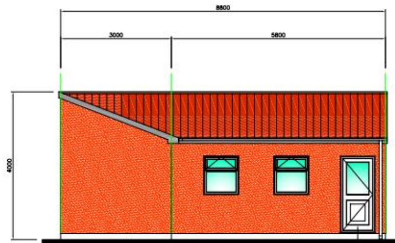
ELEVATION LOOKING SOUTHWEST
