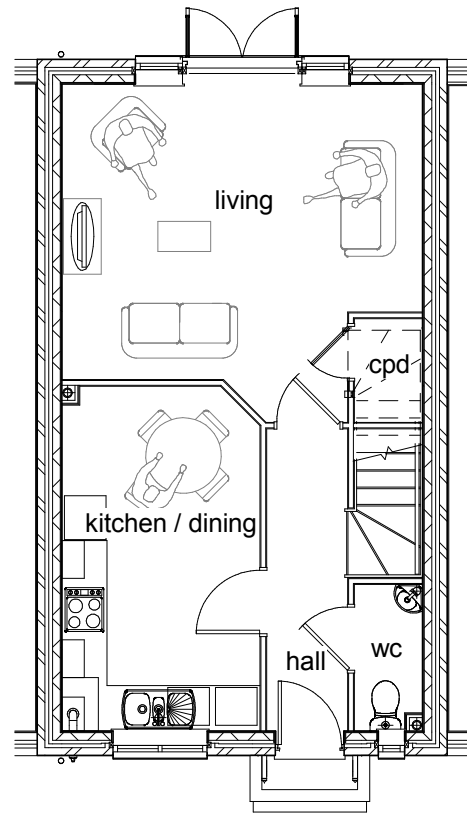
1 Ground Floor 1 : 100
