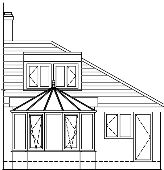
Rear Elevation
