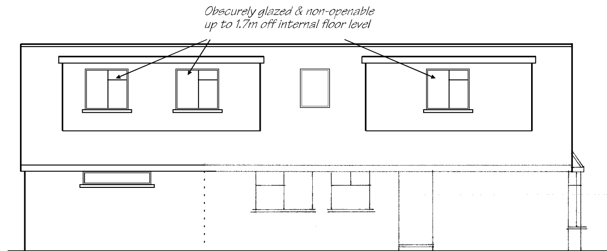
Proposed SW/Side Elevation
