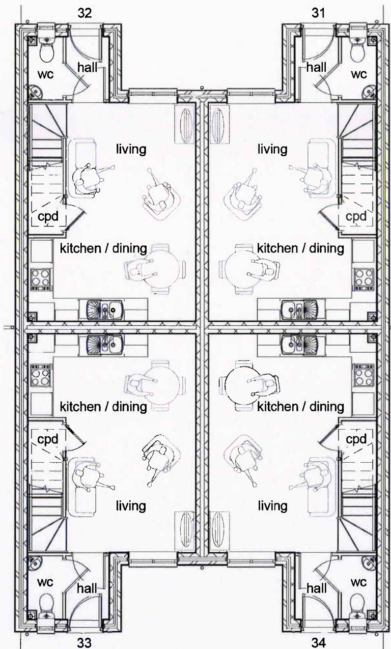
1 Ground Floor
