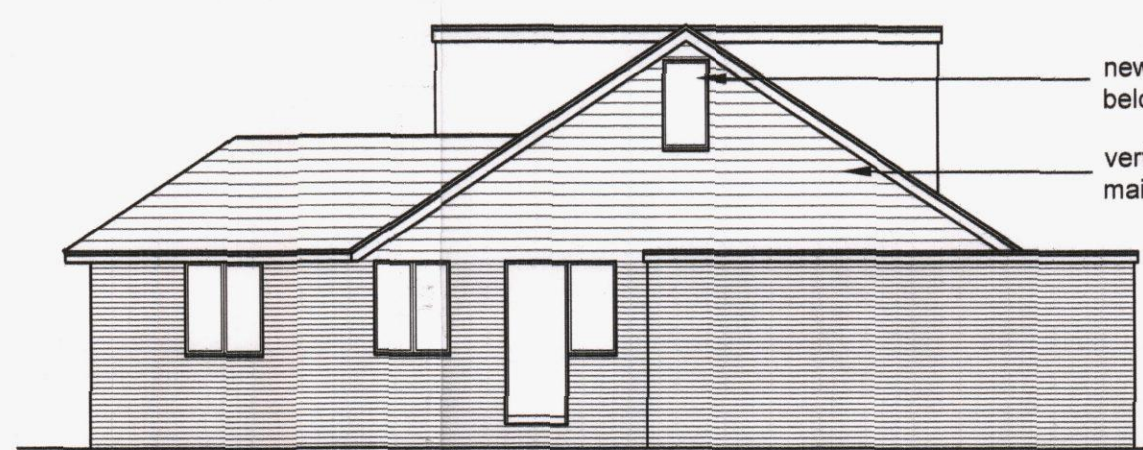
proposed north elevation 1:100
