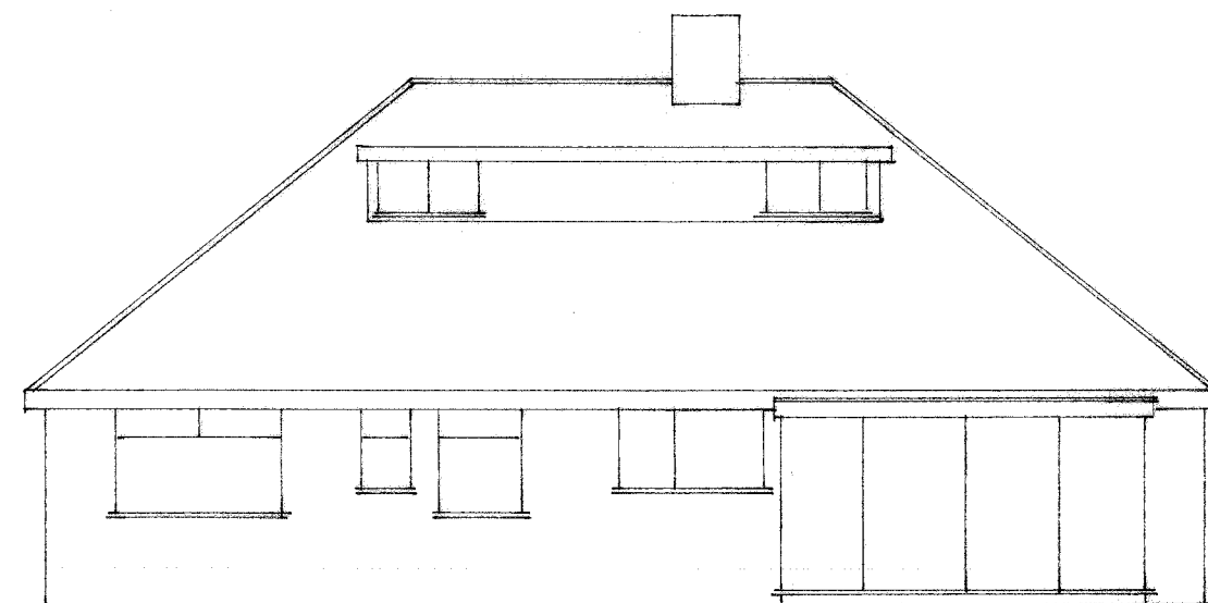
Existing NE/Rear Elevation
