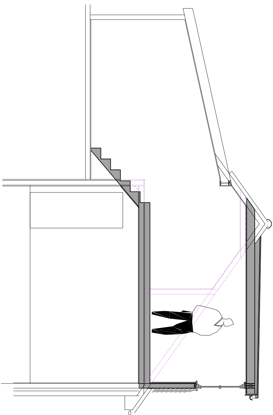
Typical Section (1:50)
