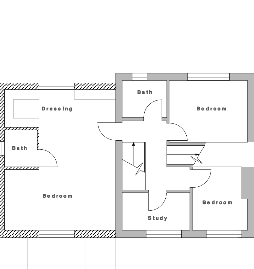
Proposed First Floor at 1:100 scale
