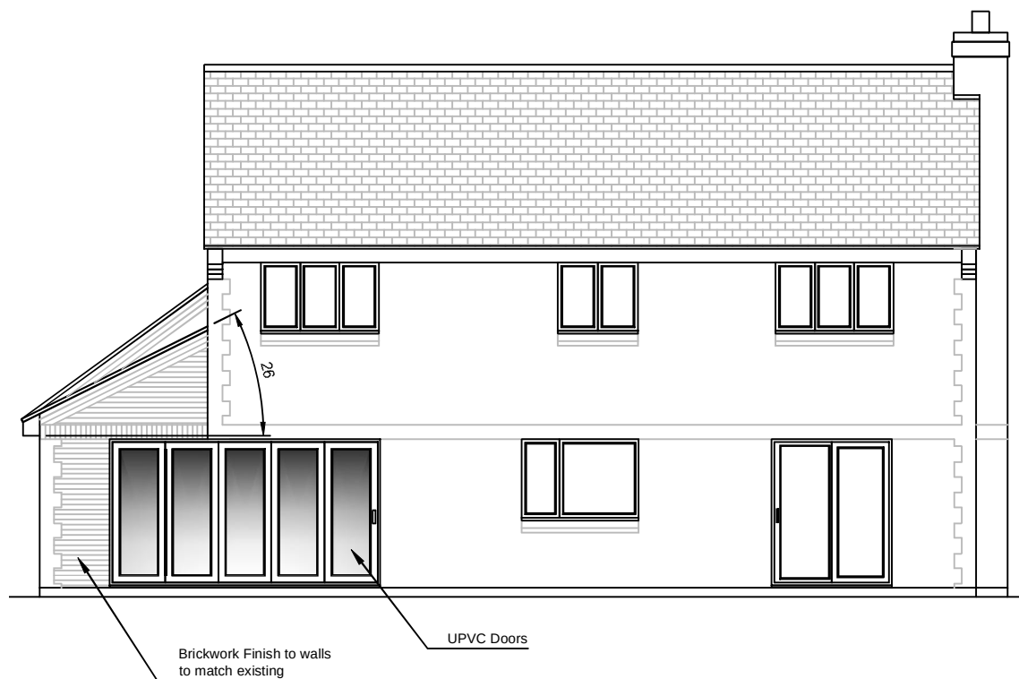
Rear Elevation
