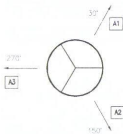
PROPOSED UPPER ANTENNA LAYOUT 1:25
