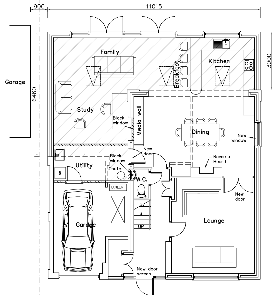
GROUND
