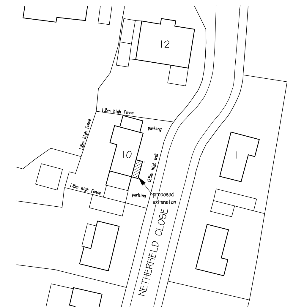
Site Plan 1 to 500
