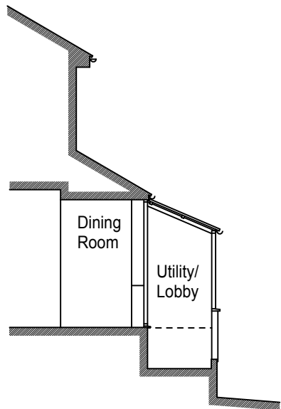
Existing Section A-A
