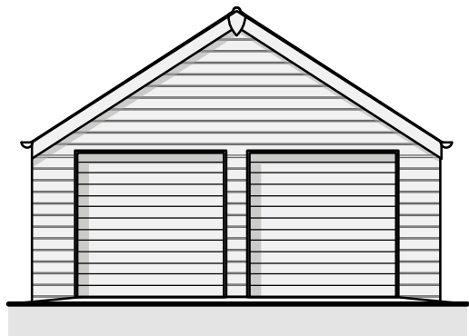
Front (West) Elevation Scale 1:100
