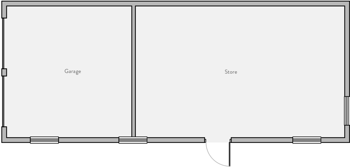
Ground Floor Plan Scale 1:100
