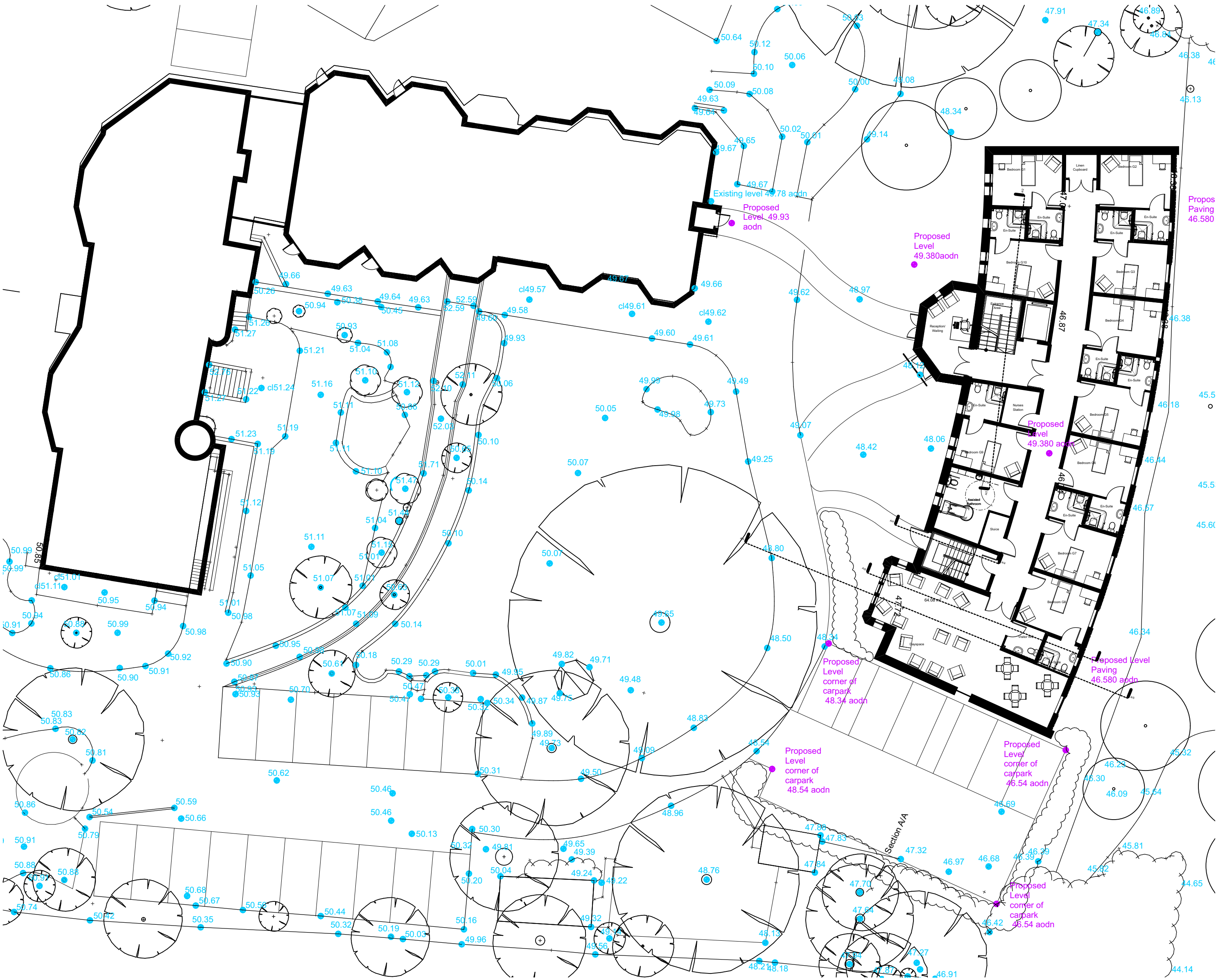
1. Ground Floor Plan 1:200
