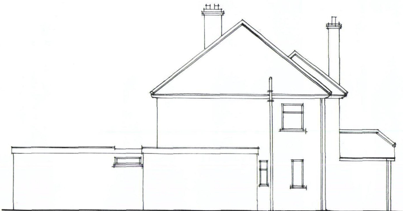
existing front elevation (SOUTH) (EXISTING COURTYARD WALL SHOWN DOTTED)
