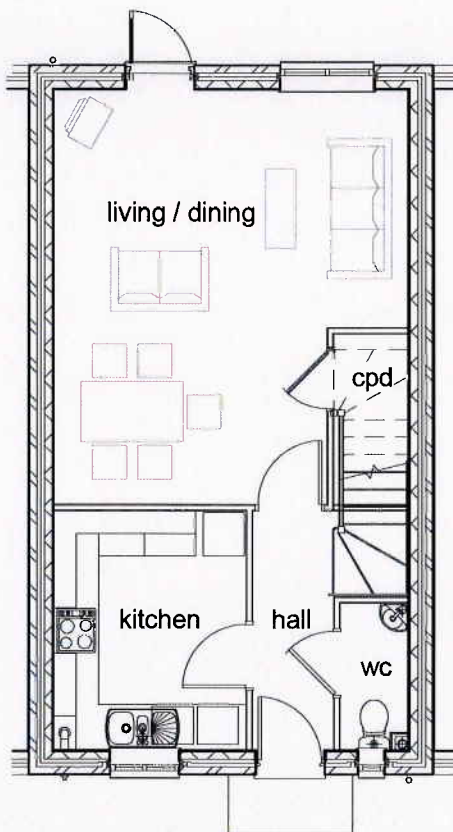
1 Ground Floor 1 : 100
