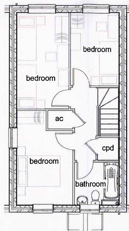
2 First Floor 1 : 100
