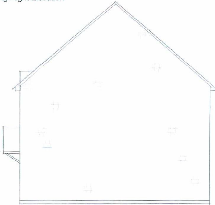
Existing Right Elevation
