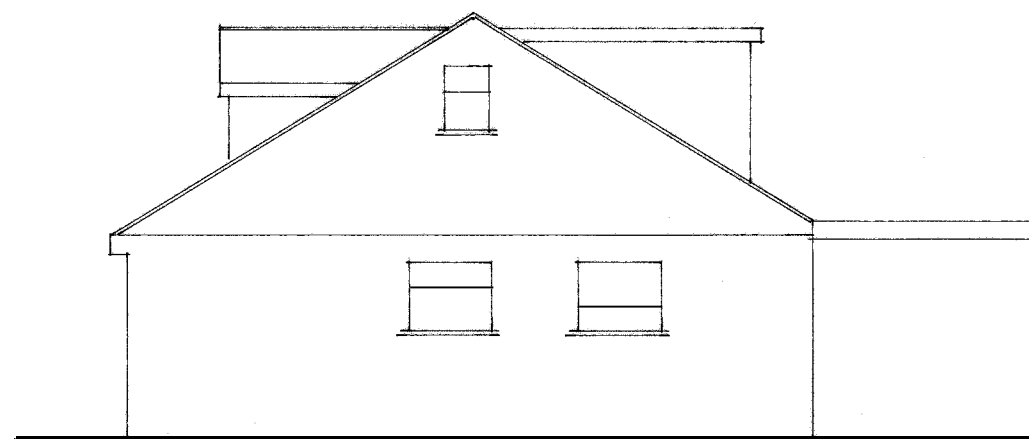
Proposed SW/Side Elevation
