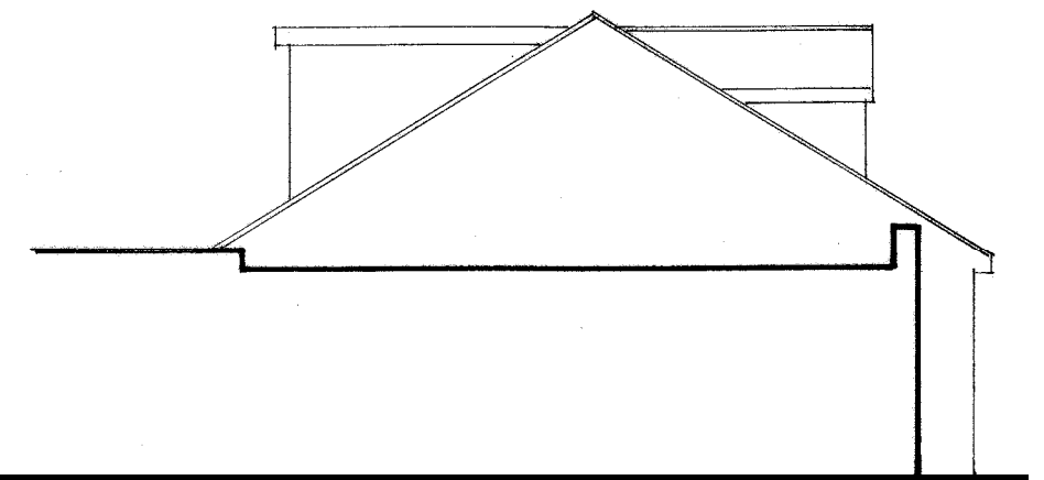
Existing NE/Side Elevation
