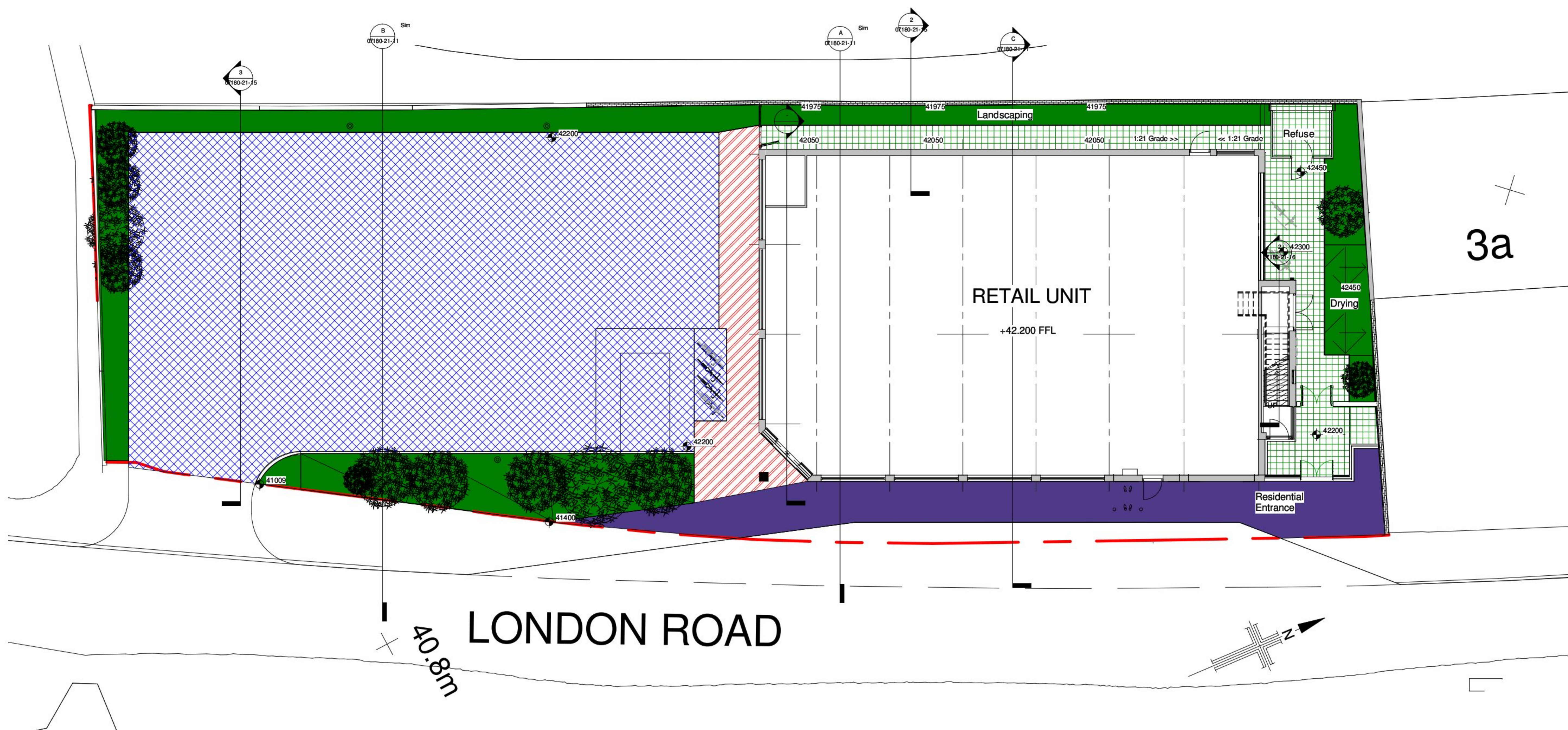
HARD LANDSCAPING PLAN 1 : 100
