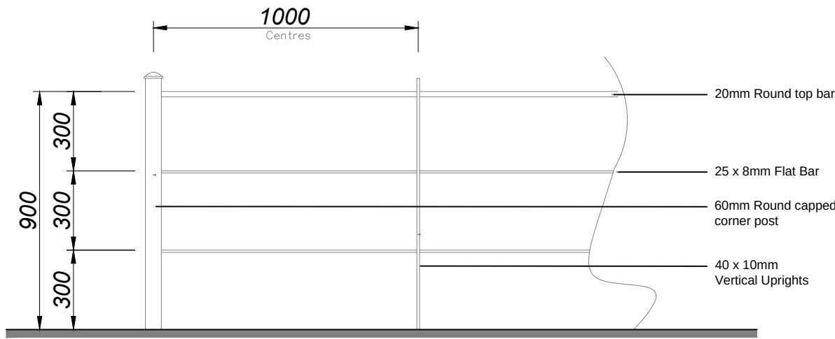
900mm ESTATE STYLE METAL RAILINGS 1:20
