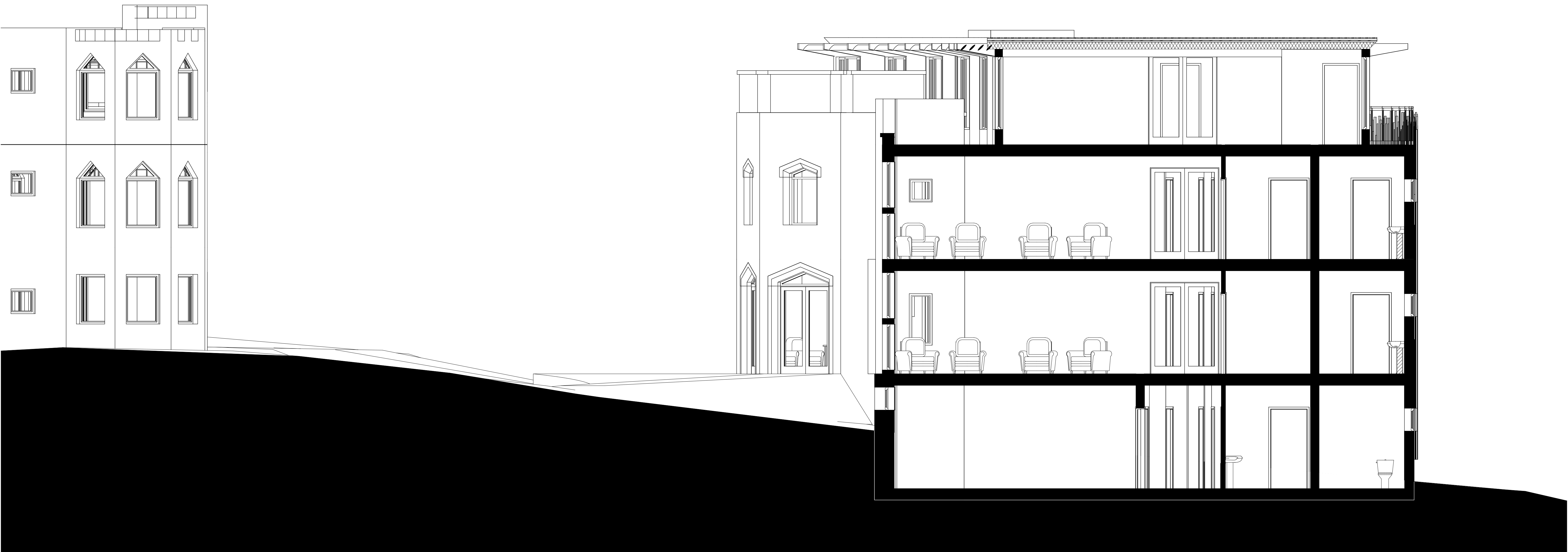
Section C-C
