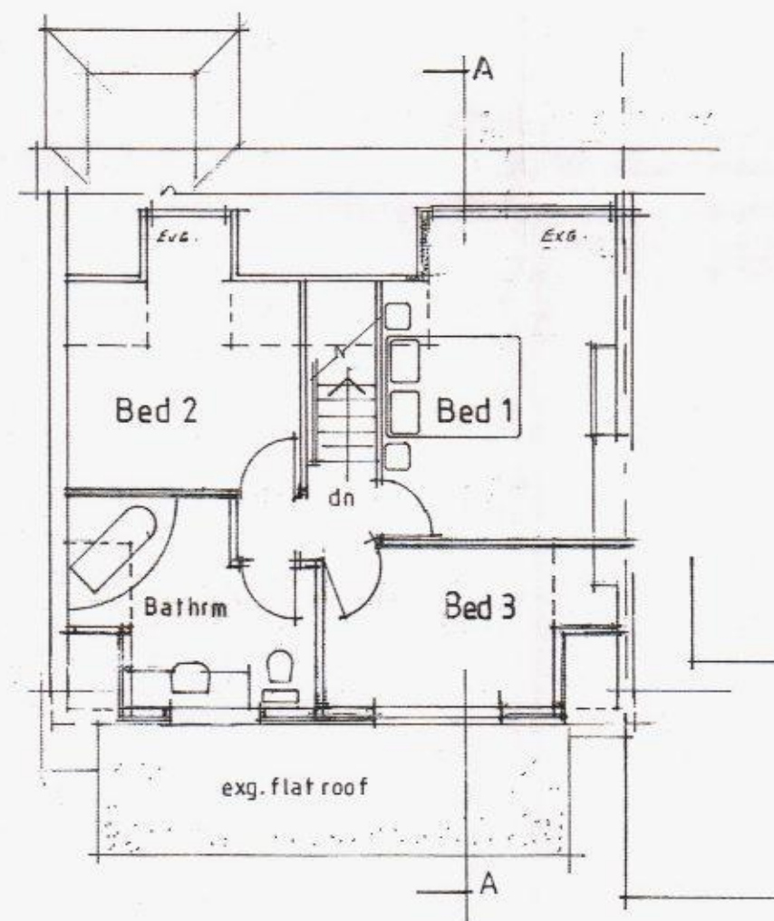
First Floor
