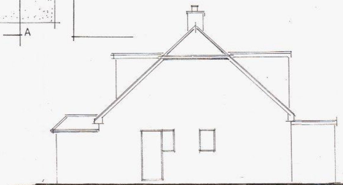
North elevation
