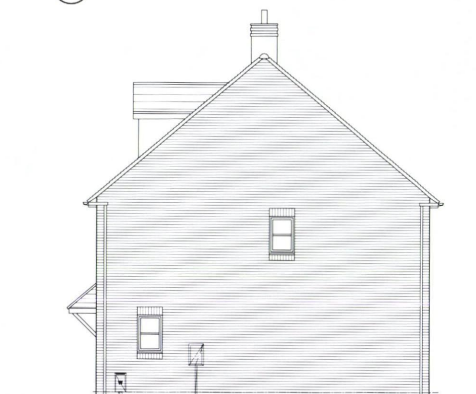
02 38 Side Elevation
