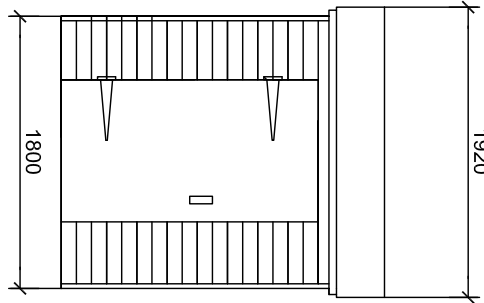
FRONT ELEVATION (B)
