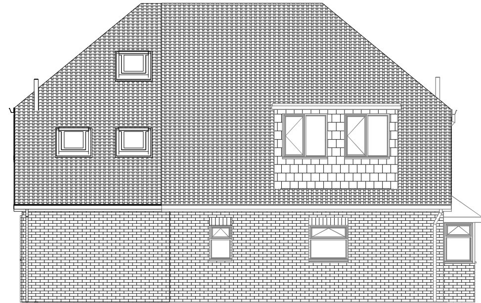
ELEVATION SOUTH EAST 1 : 100
