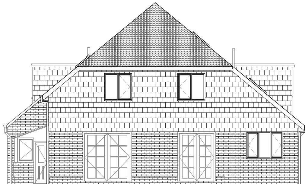
ELEVATION SOUTH WEST 1 : 100
