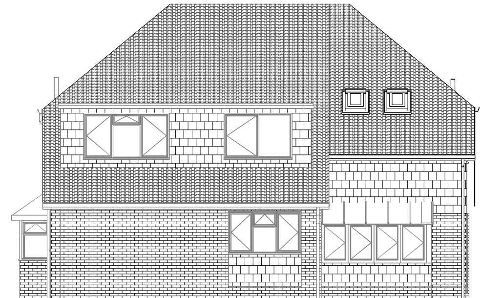
ELEVATION NORTH WEST 1 : 100
