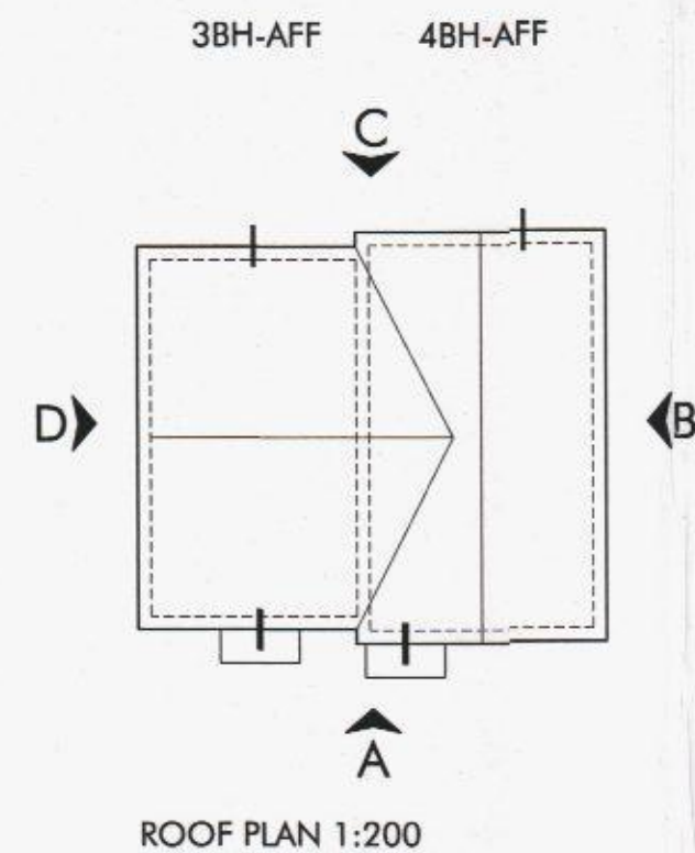
ROOF PLAN 1:200
