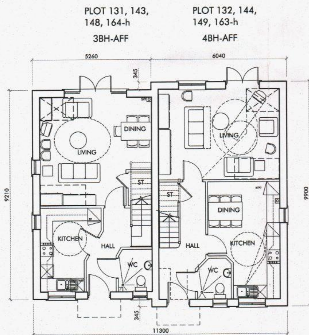
GROUND FLOOR
