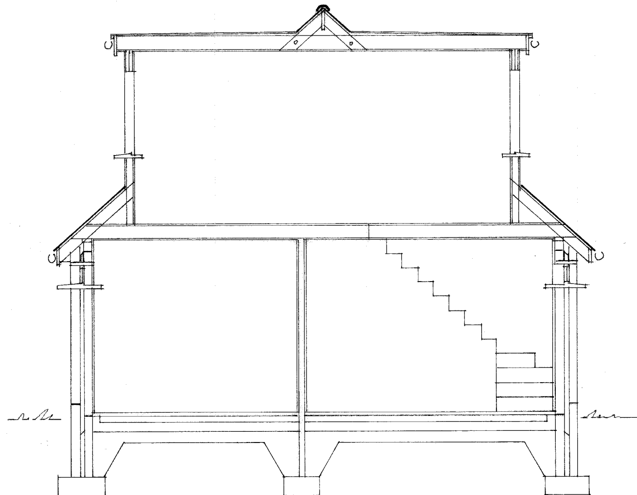
Proposed Cross-Section
