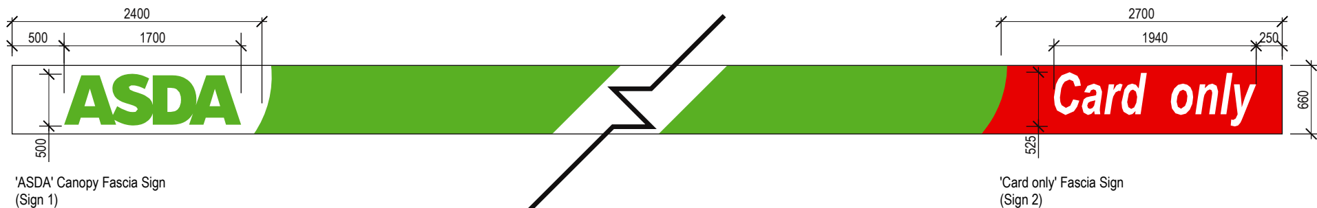
Side Elevations
