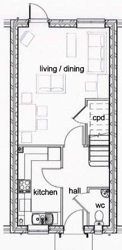
1 Ground Floor 1 : 100
