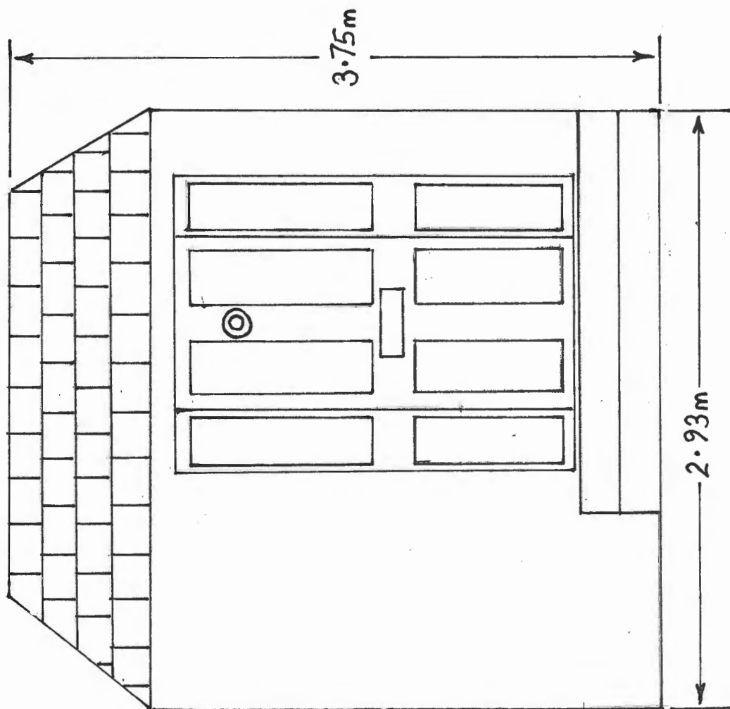
FRONT ELEVATION
