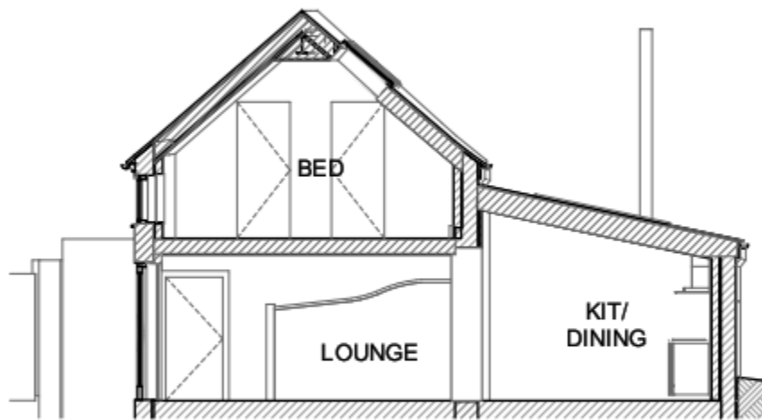
CROSS SECTION LOOKING TO WEST: AS PROPOSED
