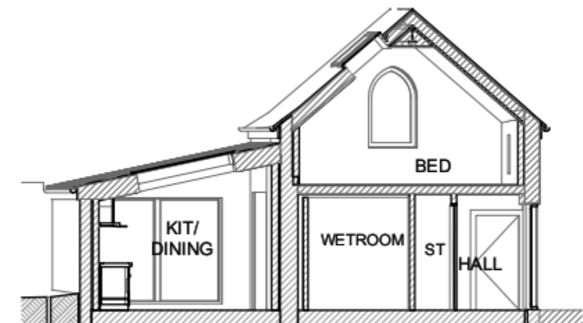
CROSS SECTION LOOKING TO EAST: AS PROPOSED
