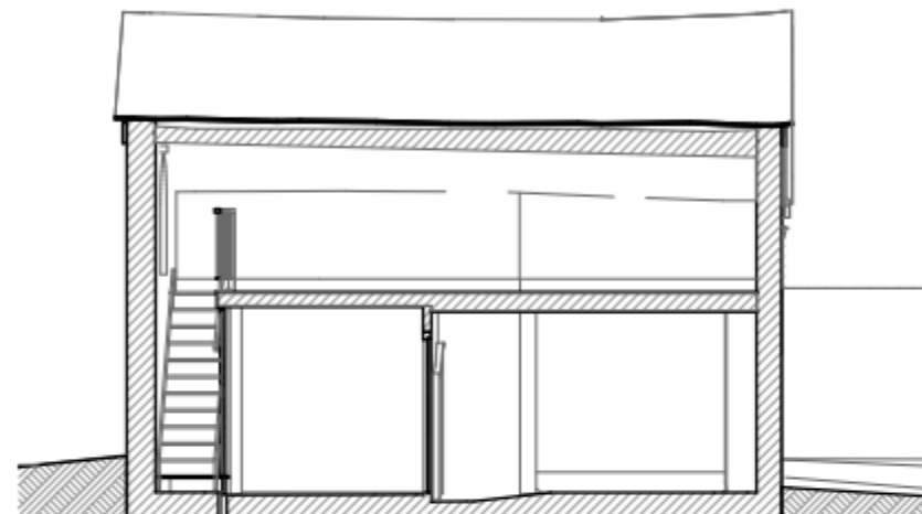
LONG SECTION LOOKING TO NORTH: AS EXISTING
