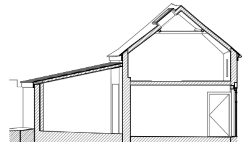
CROSS SECTION LOOKING TO EAST: AS EXISTING
