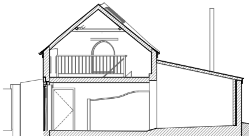
CROSS SECTION LOOKING TO WEST: AS EXISTING
