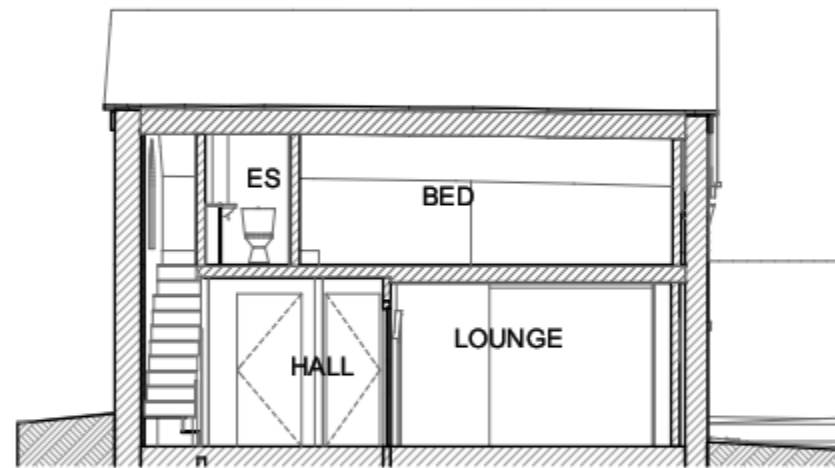
LONG SECTION LOOKING TO NORTH: AS PROPOSED
