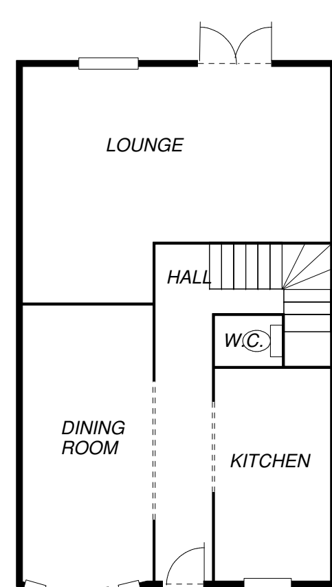
PROPOSED PLAN VIEW
