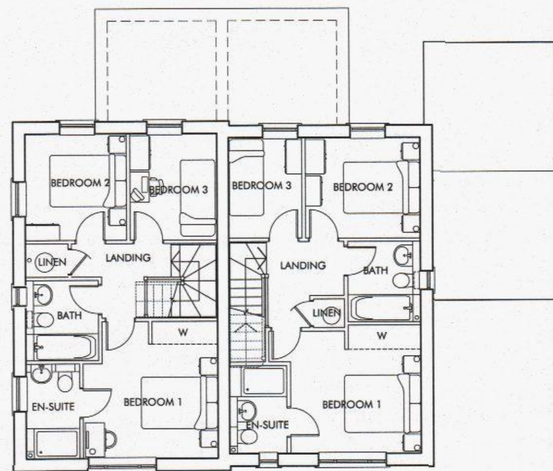
FIRST FLOOR
