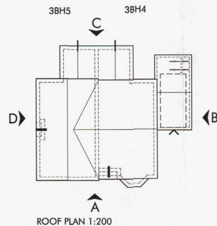
ROOF PLAN 1:200
