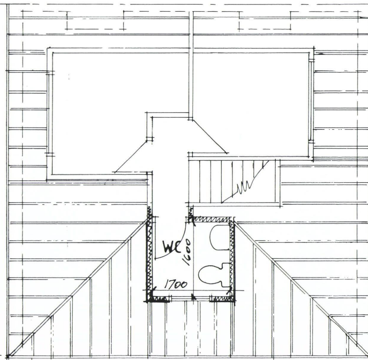
First Floor Plan - proposed
