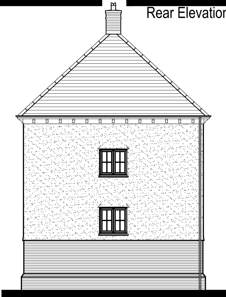
Side Elevation
