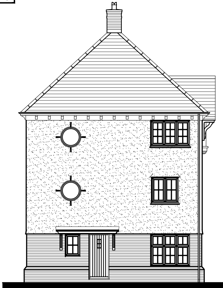
Front Elevation
