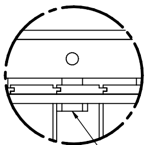
DETAIL A Top Removable Panel notched out for hasp to slide past
