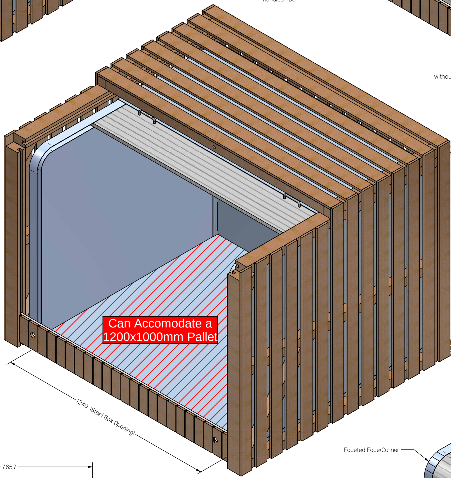
with Tambour Door Open
