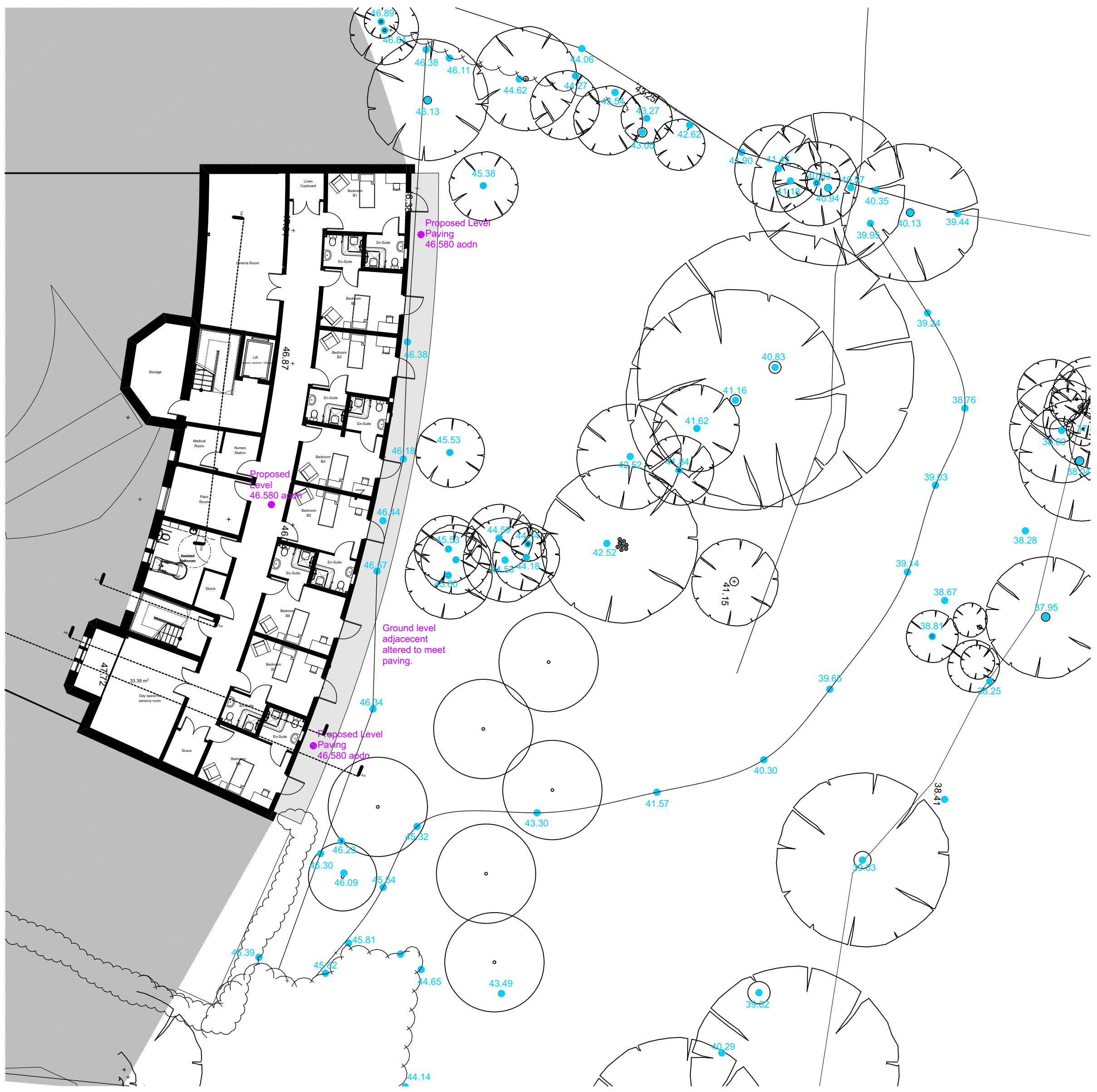
0. Basement Plan 1:200
